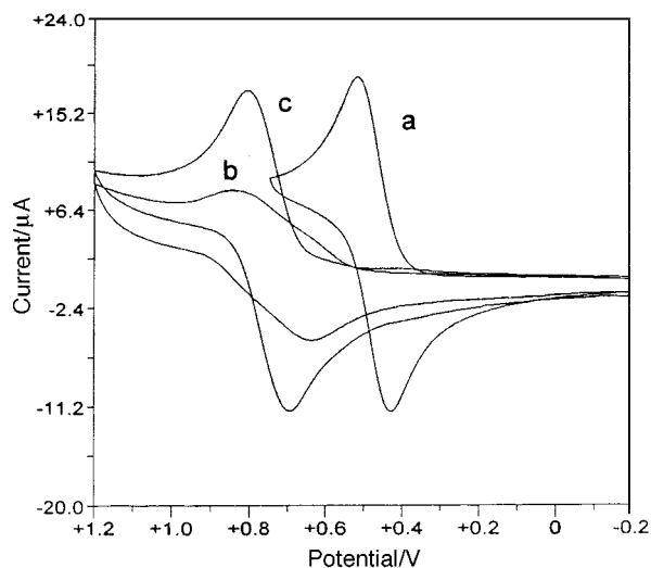
Fig. 1 Cyclic voltammetric responses recorded at a glassy-carbon electrode on \text{CH}_2\text{Cl}_2 solutions containing [\text{NBu}_4][\text{PF}_6] ( 0.2 \text{ mol dm}^{-3} ) and (a) \text{L}^1 ( 1.0 \times 10^{-3} \text{ mol dm}^{-3} ), (b) complex 1 ( 0.4 \times 10^{-3} \text{ mol dm}^{-3} ), (c) complex 2 ( 0.8 \times 10^{-3} \text{ mol dm}^{-3} ). Scan rate 0.05 \text{ V s}^{-1} .
