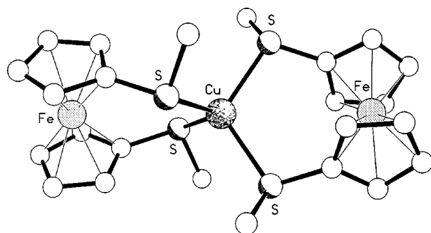
Fig. 3 The molecular structure of one of the two 50% orientations of the S_4 -symmetric cation present in the structure of complex 5 . The Cu–S and S–C 5 bond lengths are 2.331(2) [2.327(2)] and 1.746(5) [1.755(6) Å] respectively. The associated bite and interligand S–Cu–S angles are 112.28(10) [112.33(10)] and 108.08(5) [108.06(5)°] respectively; the Cu–S–C 5 angles are 109.2(3) [109.6(3)°], the number in [] referring to the alternative orientation present in the crystal.
