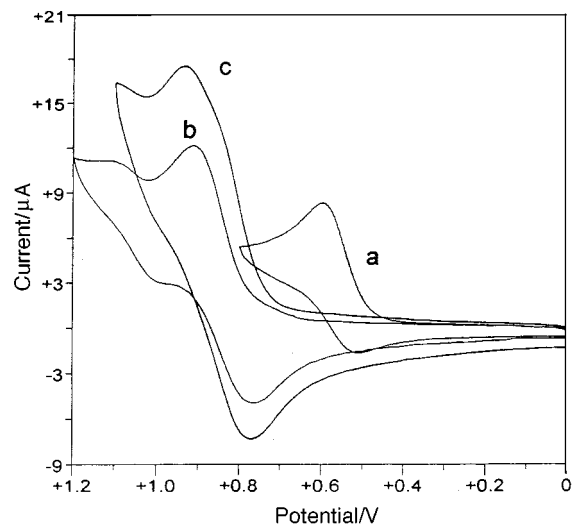
Fig. 2 Cyclic voltammetric responses recorded at a glassy-carbon electrode on \text{CH}_2\text{Cl}_2 solutions containing [\text{NBu}_4][\text{PF}_6] ( 0.2 \text{ mol dm}^{-3} ) and (a) \text{L}^2 ( 0.8 \times 10^{-3} \text{ mol dm}^{-3} ), (b) complex 3 ( 1.0 \times 10^{-3} \text{ mol dm}^{-3} ), (c) complex 4 ( 0.9 \times 10^{-3} \text{ mol dm}^{-3} ). Scan rates: (a, c) 0.05 ; (b) 0.1 \text{ V s}^{-1} .
